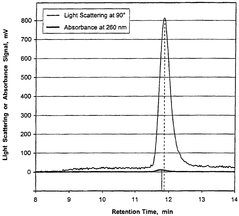
Figure 1 Detection of 4.4 \times 10^9 Adenovirus Particles by Ion-Exchange Chromatography Using Light Scattering at 90^\circ and Absorbance at 260 nm
